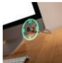
ACC0036 This one is displaying time as it plays, you can also display your logo or slogan. Material: TPU, SS304 Fan diameter: 8.8cm Length: 40 cm
